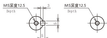
附带键 Shaft with key
